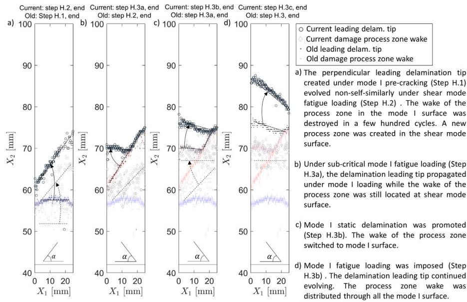
Fig. 14. Overview of the fatigue benchmark results.
