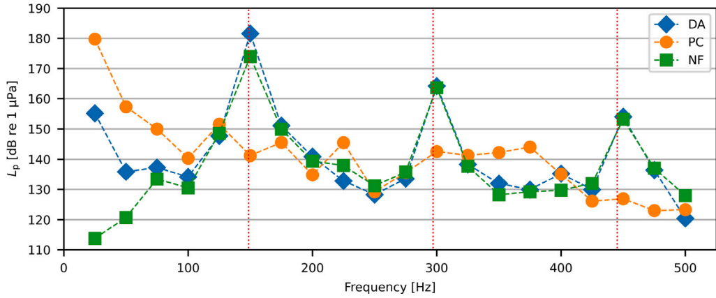
Fig. 9. Sound pressure levels for the three cases at r = 50 m and z = 7 m and for a driving depth z_2 = 14 m.
