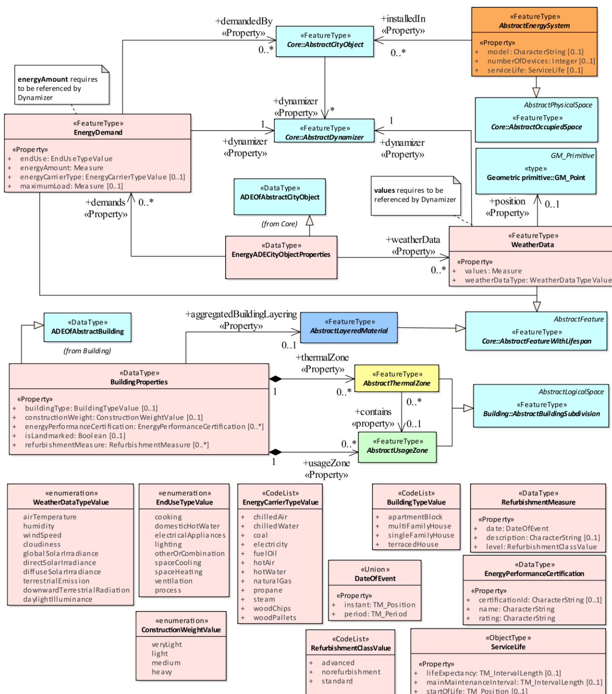
Figure 10. The Core module of the Energy ADE for CityGML 3.0.
