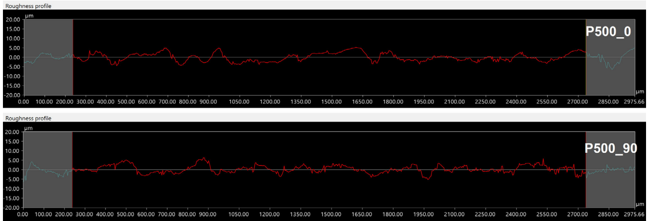
FIGURE 6 Surface roughness of the cement sample after grinding with grit paper P500 at 2 orientations.
