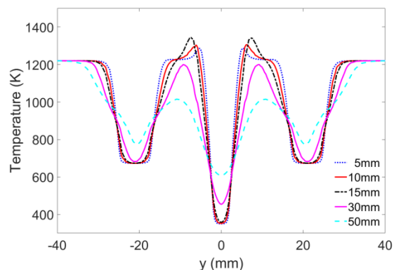
Fig. 6. Mean temperature profiles near nozzle exit.
