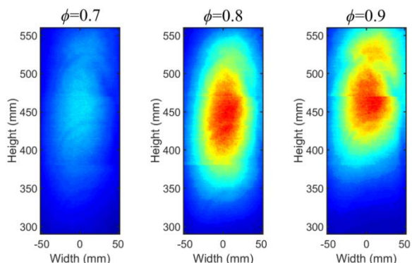
Fig. 4. Mean OH* chemiluminescence at different equivalence ratios.
