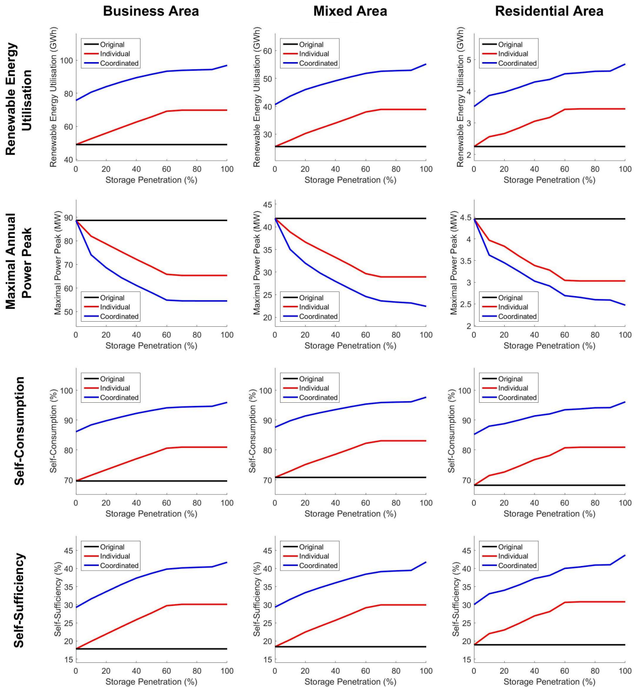
Fig.3. The impact of storage on four metrics assessing the local ability to integrate renewable resources in three representative urban areas. The four metrics are shown in subsequent rows: renewable energy utilisation (upper row), maximal annual power peak (second row), renewable energy self-consumption (third row), and area self-sufficiency (bottom row). The three representative areas are shown in three columns: business area (left), mixed area (centre), and residential area (right). Each subplot shows the impact of increasing storage penetration (from 0% to 100% of consumers having their own storage units) for three scenarios: original scenario (no storage, individual PV), individual scenario (individually used storage and PV) and coordinated scenario (coordinated use of storage and PV). The original scenario is shown as a reference. For all plots and scenarios, the PV penetration is kept constant at 50% of the consumers having their own installation. The noise is attributed to variations in PV and storage sizes, which result from the random assignment and corresponding sizing of PV and storage systems. Note that in each simulation the original, individual and coordinated scenarios are calculated for the same set of PV and storage capacity. The results shown are averages of 30 simulations.
