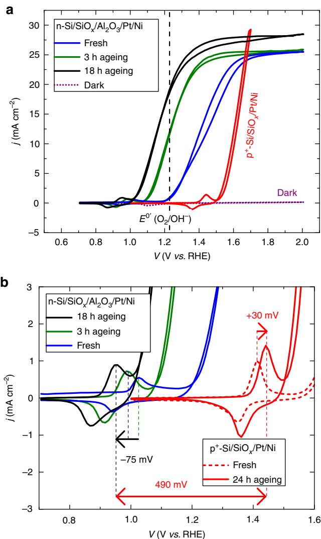
Figure 2 | Cyclic voltammtries. (a) Three-electrode (photo) current density versus applied voltage ( j - V ) curves of \text{n-Si}/\text{SiO}_{x,\text{RCA}}/\text{Al}_2\text{O}_3/\text{Pt}/\text{Ni} photoanode during ageing in 1 M KOH under simulated AM1.5 illumination. A total of three illuminated voltammetry scans are shown: one for initial fresh sample (blue line), one after 3 h (green line) and one after 18 h (black line) of ageing in the electrolyte. The dark voltammetry scan of the \text{n-Si}/\text{SiO}_{x,\text{RCA}}/\text{Al}_2\text{O}_3/\text{Pt}/\text{Ni} is shown as the dotted purple line. For comparison, the j - V behaviour of the non-photoactive \text{p}^+-\text{Si}/\text{SiO}_{x,\text{RCA}}/\text{Pt}/\text{Ni} is shown (red line). The black vertical dashed line indicates the potential for water oxidation, E^0(\text{O}_2/\text{OH}^-) . (b) The magnification of Fig. 2a, showing the shift of the redox peaks of Ni over the course of 18 h.
