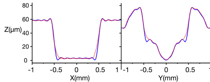
Fig. 2. Two cross sections or surface profiles measured orthogonally from a unit cell of the manufactured 8-pixel grating (dashed), together with the designed profiles (solid), for comparison (corresponding to the 3D profile shown in the middle of the Fig. 1). Here Z is the vertical direction of the grating.
