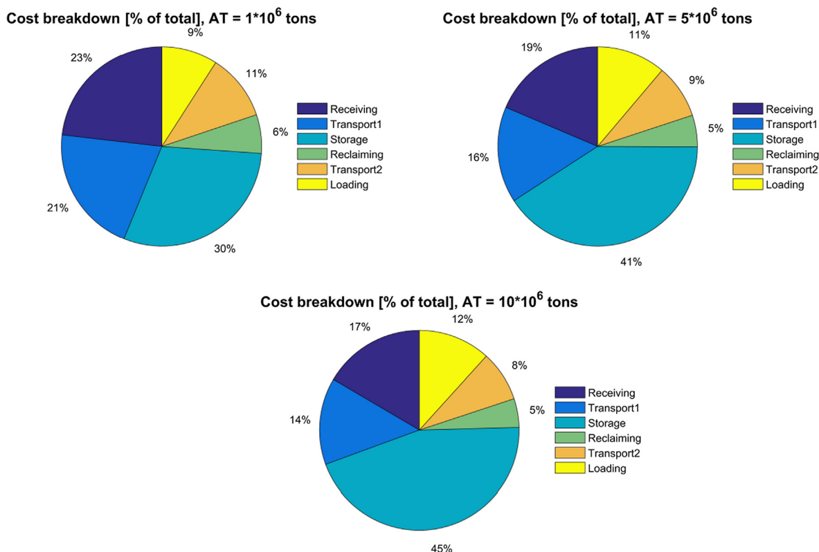
Fig. 5. Total cost breakdown (1, 5 & 10 Mt throughput terminals).
