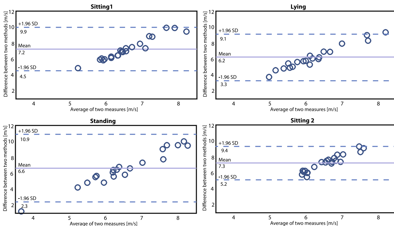
Fig. 3 Bland–Altman plots of PWV_{complior} and PWV_{biopac} by the four positions. The dotted lines represent the 95% limits of agreement and the straight mean difference (bias) between PWV_{complior} and PWV_{biopac}
