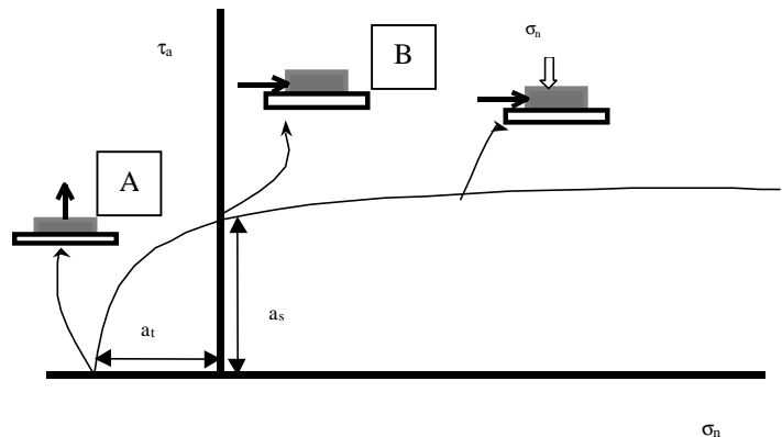
Figure 1 : Empirical graph of the adhesion model. Adhesive shear strength ( \tau_a ) versus applied normal stress ( \sigma_n ).
