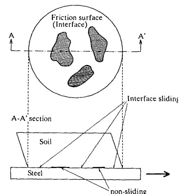
Figure 2 : Mode 3. Partial sliding at soil steel interface (Tsubikahara, 1993)
