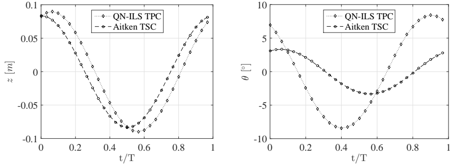
Figure 8: Aitken time step and QN-ILS time periodic solution for z and \theta as a function of the normalized time, t/T , for the 2-DoF problem, \omega = 4\pi .
