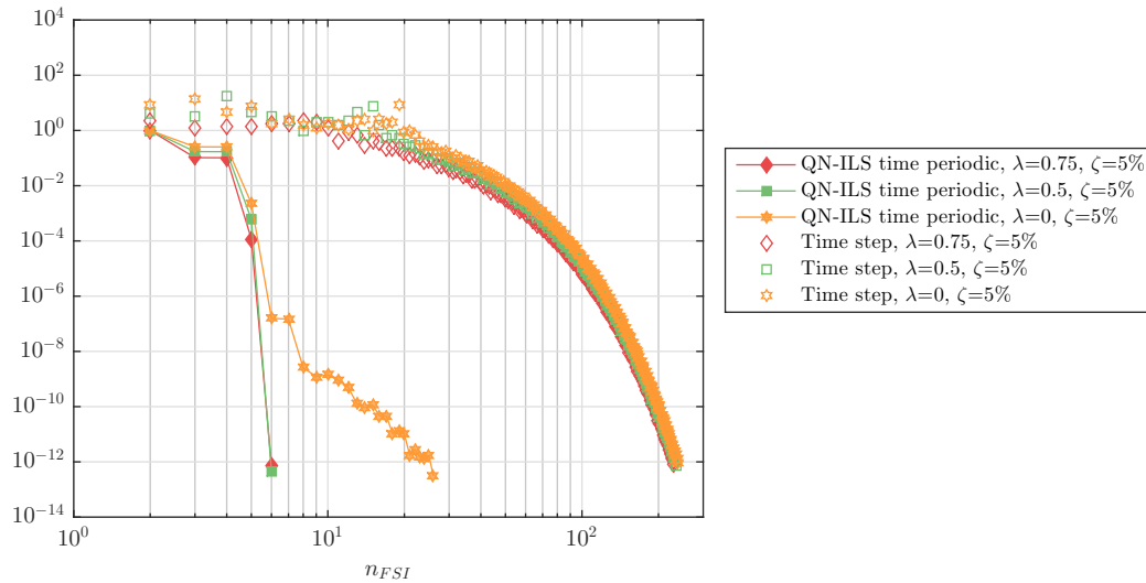
Figure 4: Convergence behaviour of the time step and QN-ILS time periodic coupling for the 1-DoF plunging problem for different fluid added mass fractions.
