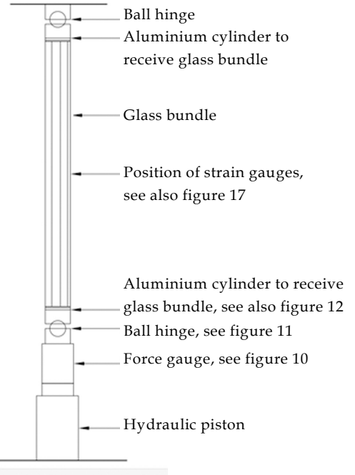
Figure 14: Diagram of the test setup
