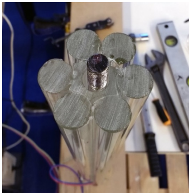
Figure 4 and 5: Cross-section of the bundles
