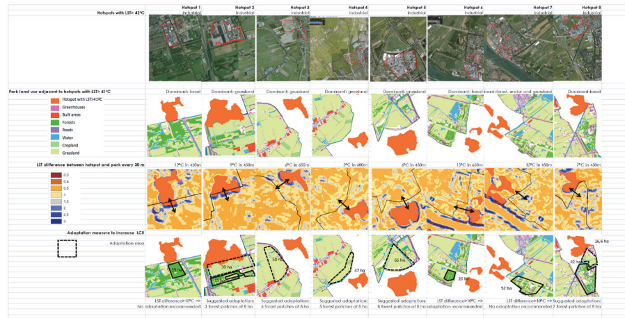
FIGURE 4.3 Diagnosis and adaptation design for hotspots with an LST > 42°C (Echevarria Icaza et al., 2016a).
