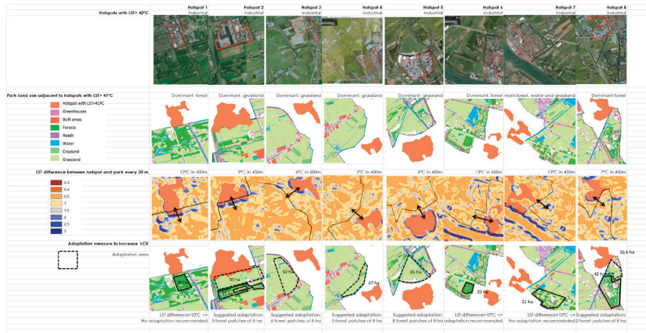
FIGURE 7.18 Diagnosis and adaptation design for hotspots with an LST > 41°C.
