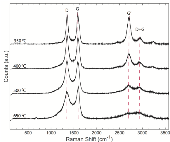
Fig. 7. Raman spectra of CNTs grown on 5 nm Co at four different growth temperatures. To obtain insights about CNT properties like purity and structural quality, the ( I_{D/G} ) ratio is calculated. The ( I_{D/G} ) ratio decreases as the CNT growth temperature increases.
