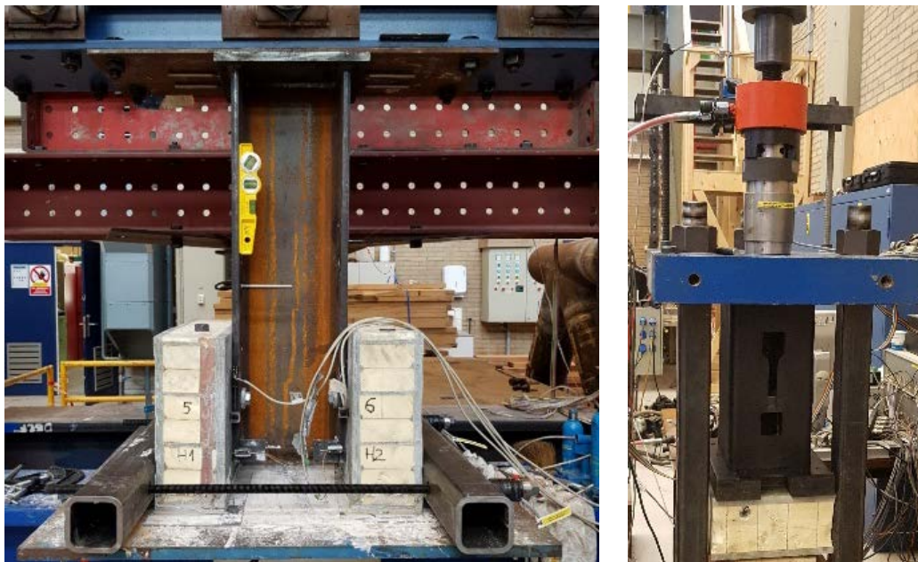
Figure 1. Push-out (left) and pull-out (right) tests
