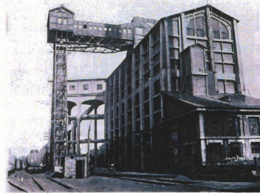
Figure 30: Reinforced concrete construction of the Blast furnace of the Coke-chemical plant in Tscheglovo (Kemerovo), designed by Olivier Piëtte, 1916.
