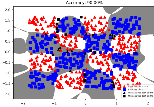
(a) Nonlinear WLTSVM ( c = 2^{-3}, k = 8, \sigma = 2^0 )
