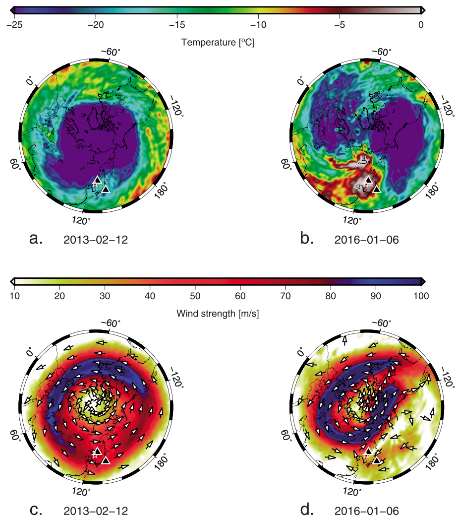
Figure 2. The wind and temperature at 1.5 hPa ( \sim 45 km) from ECMWF atmospheric specifications. IMS infrasound stations are indicated with the black triangles, being I45RU to the north of Punggye-ri (star) and I30JP to the east. The temperatures are given in (a) 2013/02/12 03:00 UTC and (b) 2016/01/06 02:00 UTC. The wind strength and direction are shown in (c) 2013 and (d) 2016.
