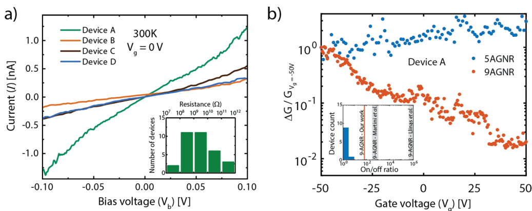
Figure 3. Electrical device characterization at room temperature. (a) I – V curves measured on four devices after transfer of the 5-AGNR at zero gate voltage. The bottom-right inset corresponds to the histograms of the low-bias resistance measured for all the 5-AGNR devices. (b) Conductance at fixed bias voltage as a function of gate voltage for the 5-AGNR (device A) and 9-AGNR.
