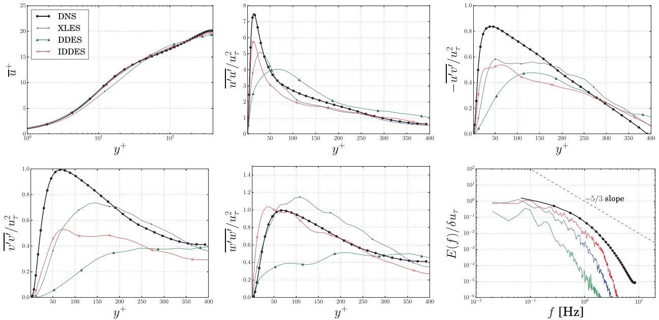
Fig. 9. Normalised mean velocity and Reynolds stress profiles and turbulence kinetic energy spectra using Hybrid models and DNS [28]. From left to right, and top to bottom \bar{u}^+ , Re_{uu} , Re_{uv} , Re_{vv} , Re_{vw} and E_{u,y^+ \approx 20}(f) .
