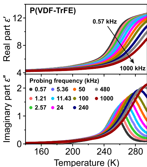
Figure 5. Temperature dependence of the real and imaginary parts of the complex dielectric permittivity of the P(VDF–TrFE) copolymer film probed at different frequencies.
