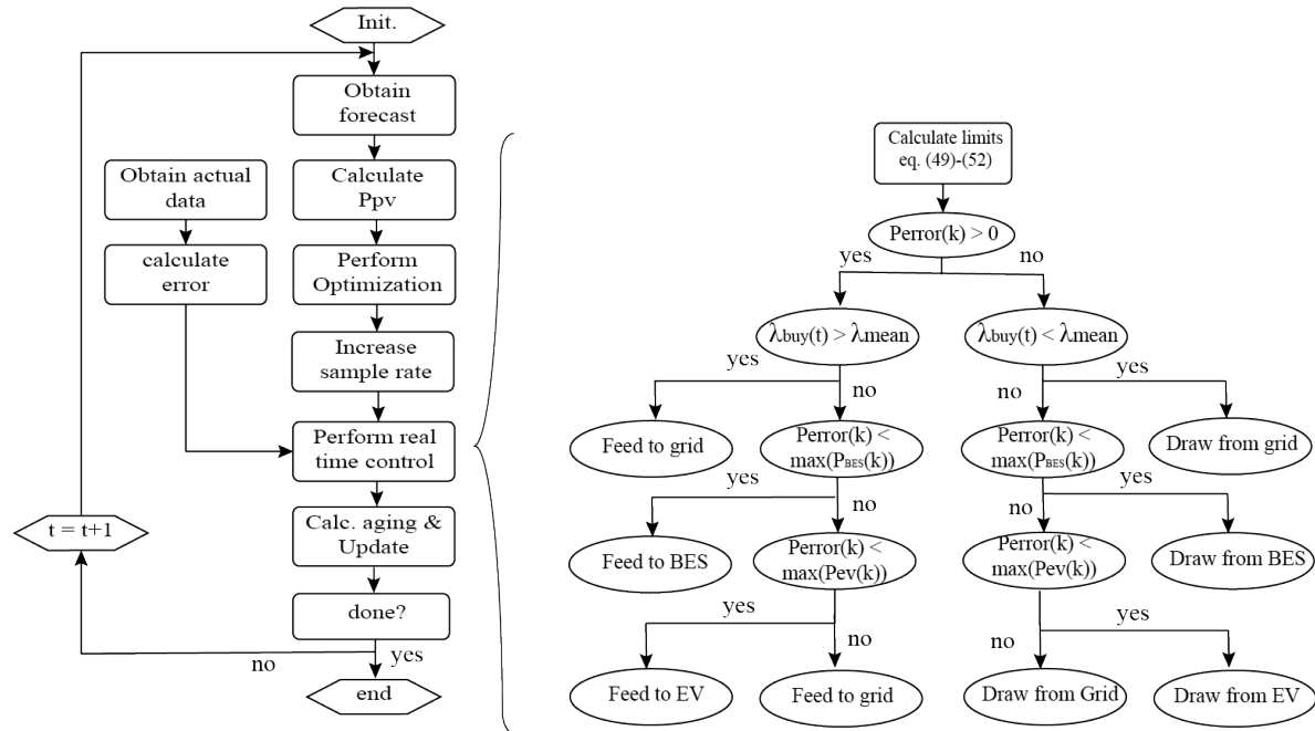
Figure 5. Moving horizon and real-time control flowchart.
