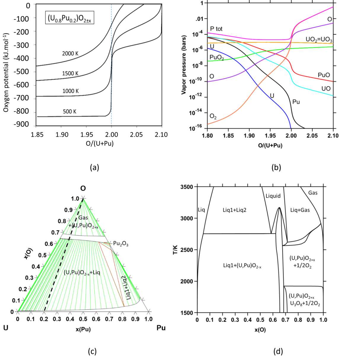
Figure 4: Calculated (a) oxygen potential of (\text{U}_{0.8}\text{Pu}_{0.2})\text{O}_{2\pm x} as function of \text{O}/(\text{U}+\text{Pu}) ratio at 500, 1000, 1500 and 2000 K ; (b) vapor pressure of the gaseous species and total pressure above (\text{U}_{0.8}\text{Pu}_{0.2})\text{O}_{2\pm x} as function of \text{O}/(\text{U}+\text{Pu}) at 2300 K ; (c) isothermal section of the U-Pu-O system at 2300 K ; (d) isopleth section of the U-Pu-O system with \text{U}/\text{Pu}=4 along the composition line reported on the isothermal section (dashed line).
