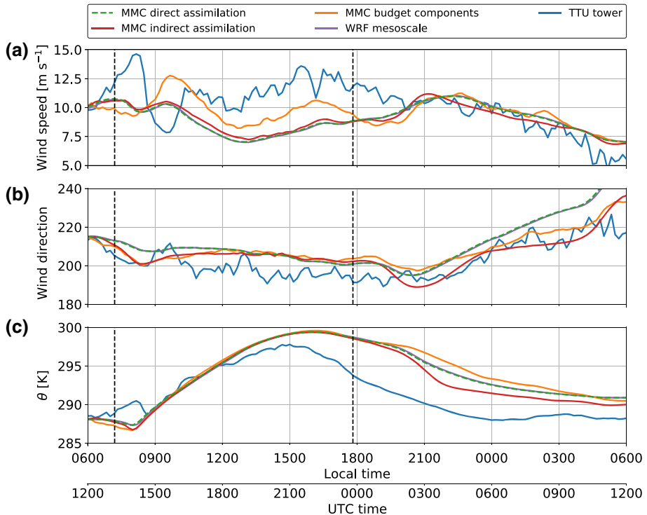
Fig. 4 Time history for 8 and 9 November 2013 at a height of 80 m of a horizontal wind speed, b wind direction, and c virtual potential temperature, comparing direct and indirect data assimilation with TTU tower observations, WRF mesoscale data, and MMC using budget components. The microscale results represent planar-averaged data. Vertical dashed black lines indicate sunrise and sunset
