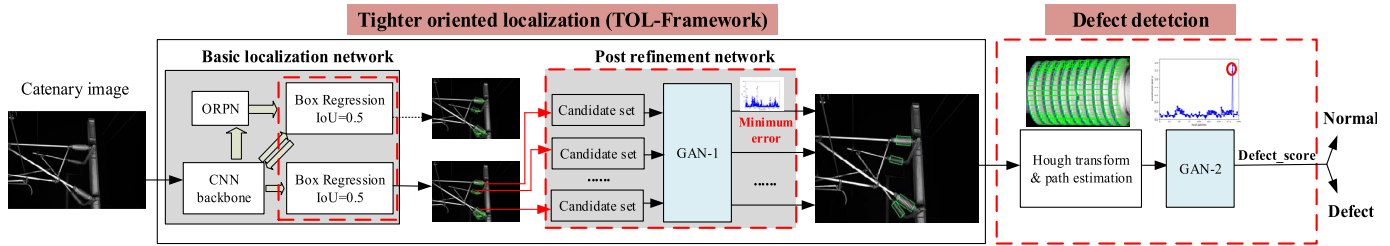
Fig. 3. Overview of the proposed insulator defect detection method.
