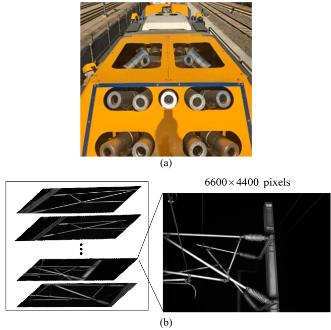
Fig. 10. Image data collection. (a) JX-300 inspection vehicle. (b) Collected catenary images.
