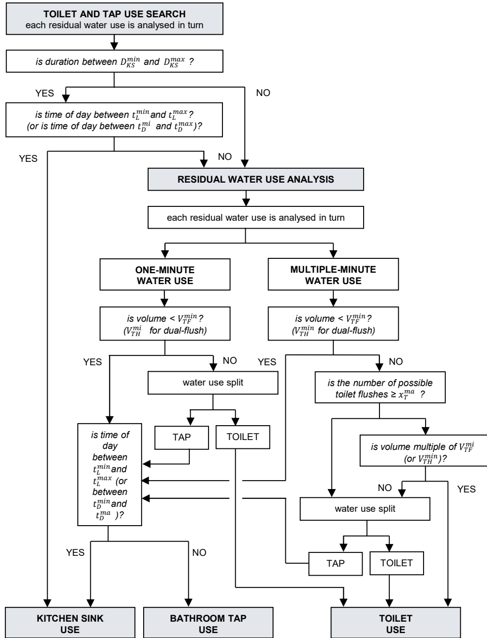
Fig. S3. Function for toilet and tap use detection ( F_{TT} ) flow chart.
