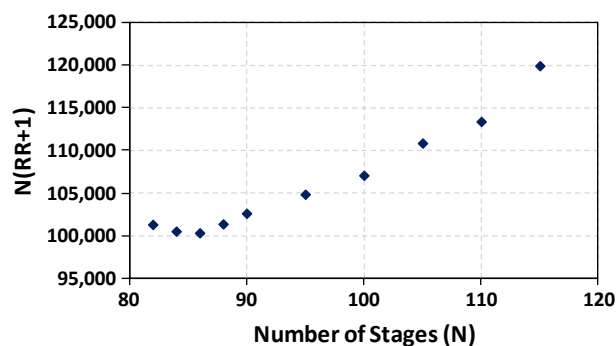
Fig. 3. Determination of the optimum number of stages for the DWC.
