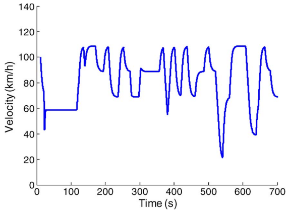
Fig. 5. Speed profile of the lead car.
