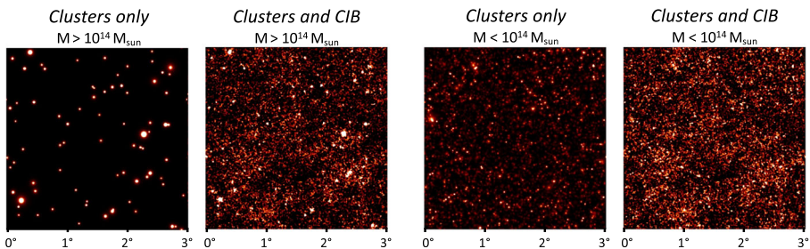
Fig. 1 Impact of the Cosmic Infrared Background (CIB) for detecting low-mass galaxy clusters at 150 GHz. Left two panels: simulated clusters of more than 10^{14} M_{\odot} , without and with 150-GHz CIB fluctuations added. Right two panels: same but with clusters of mass between 1 \times 10^{13} and 10^{14} M_{\odot} . All figures use the same color scale
