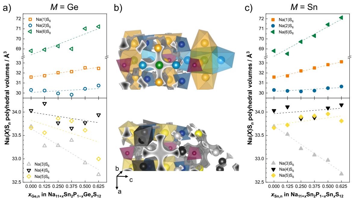
Figure 4: Volumes of the \text{Na}(X)\text{S}_n polyhedra building up the \text{Na}^+ diffusion pathways against the nominal x \text{Ge} and \text{Sn} contents in \text{Na}_{11+x}\text{Sn}_2\text{P}_{1-x}\text{M}_x\text{S}_{12} . The \text{Na}(X)\text{S}_n polyhedra in \text{b} ) with their connectivity highlighted by the surfaces of equivalent bond valence site energies representing the energetically favored \text{Na}^+ diffusion pathways. Linear fits act as guide to the eye.
