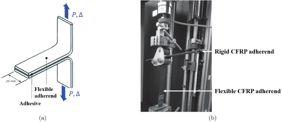
Figure 2. Schematic representation of peel testing configurations. (a) The T-peel test geometry (adopted from [25] ). (b) The Composite Peel Test (CPT) set-up (adopted from [26] ).
