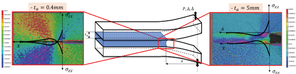
Figure 6. Adhesive thickness t_a affects the local, crack front, stress/strain field. The color map corresponds to the strain tensor shear component ( \epsilon_{xz} ) captured using the digital image correlation. Predicted distribution of the crack opening stresses \sigma_{zz} is also presented. (Courtesy of Michal K. Budzik).
