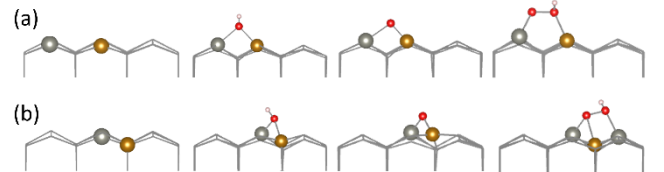
Figure 4. The atomic structures without and with OER intermediates are shown for (a) surface and (b) subsurface TM doping. The structures from left to right are in the sequence of vacant site (*), *OH, *O, and *OOH. Only the case for bridge site adsorption is shown.
