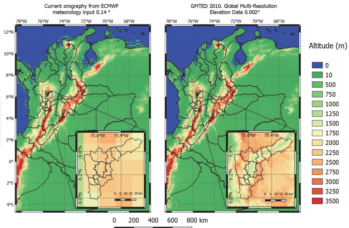
Figure 2. (Comparison between the default elevation model for LOTOS-EUROS (A) and the updated elevation model derived from the GMTED 2010 data (B). The insets illustrate the differences in elevation representation for the Aburrá Valley.
