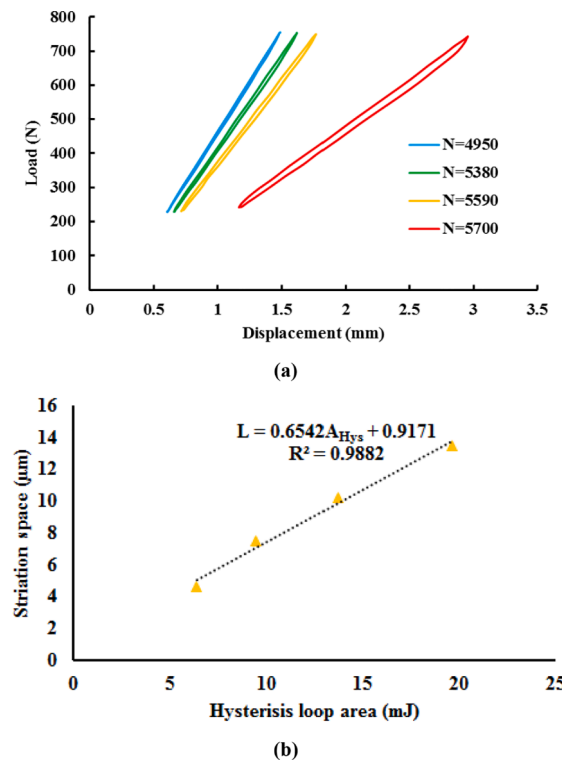
Fig. 14. (a) The hysteresis loops and (b) the relationship between the hysteresis loop area and the striations space.
