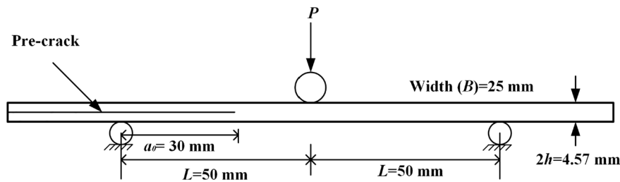
Fig. 1. The schematic of mode II test configurations.
