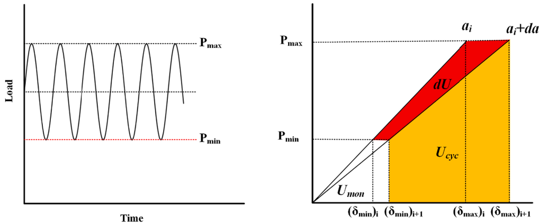
Fig. 9. Changing the potential energy due to an infinitesimal crack growth under load-control fatigue test ( a_i is the crack length at i^{th} cycle and da is the infinitesimal crack growth in one cycle).
